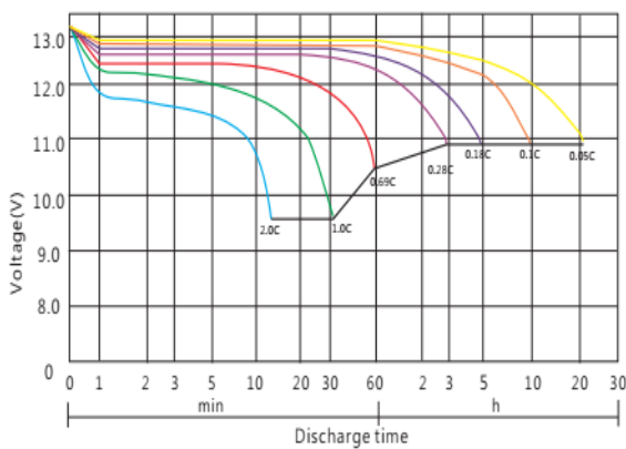
Discharge voltages vs. discharge time
