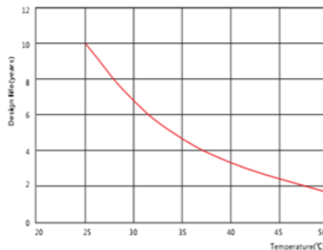
Design life vs. temperature
