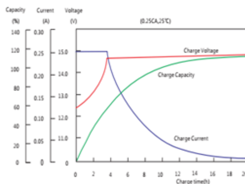
Charge capacity vs. charge time
