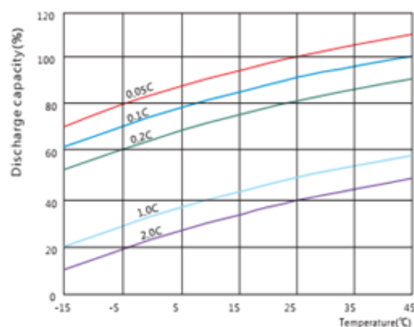
Discharge capacity vs. temperature
