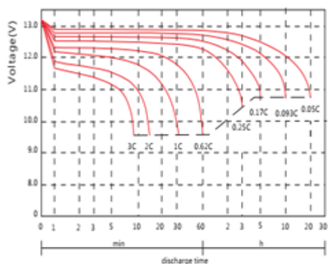
Discharge voltages vs. discharge time
