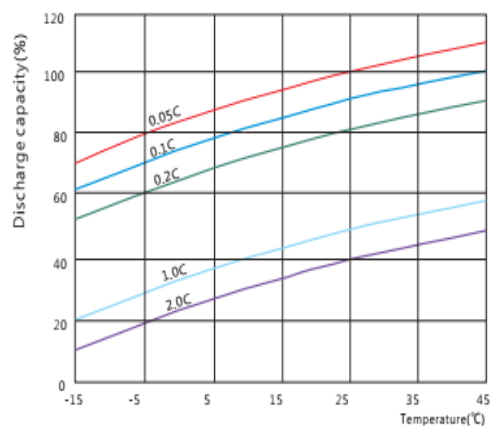
Discharge capacity vs. temperature
