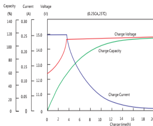
Charge capacity vs. charge time
