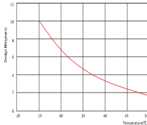
Design life vs. temperature
