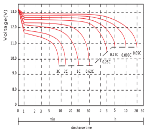
Discharge voltages vs. discharge time
